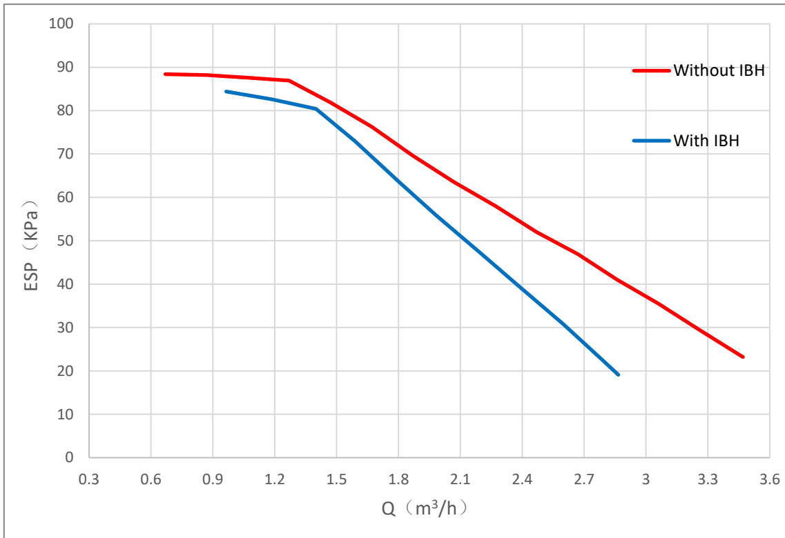
12-16kW hydronic performance 1 MUAMR-12-H14, MUAMR-14-H14, MUAMR-16-H14
