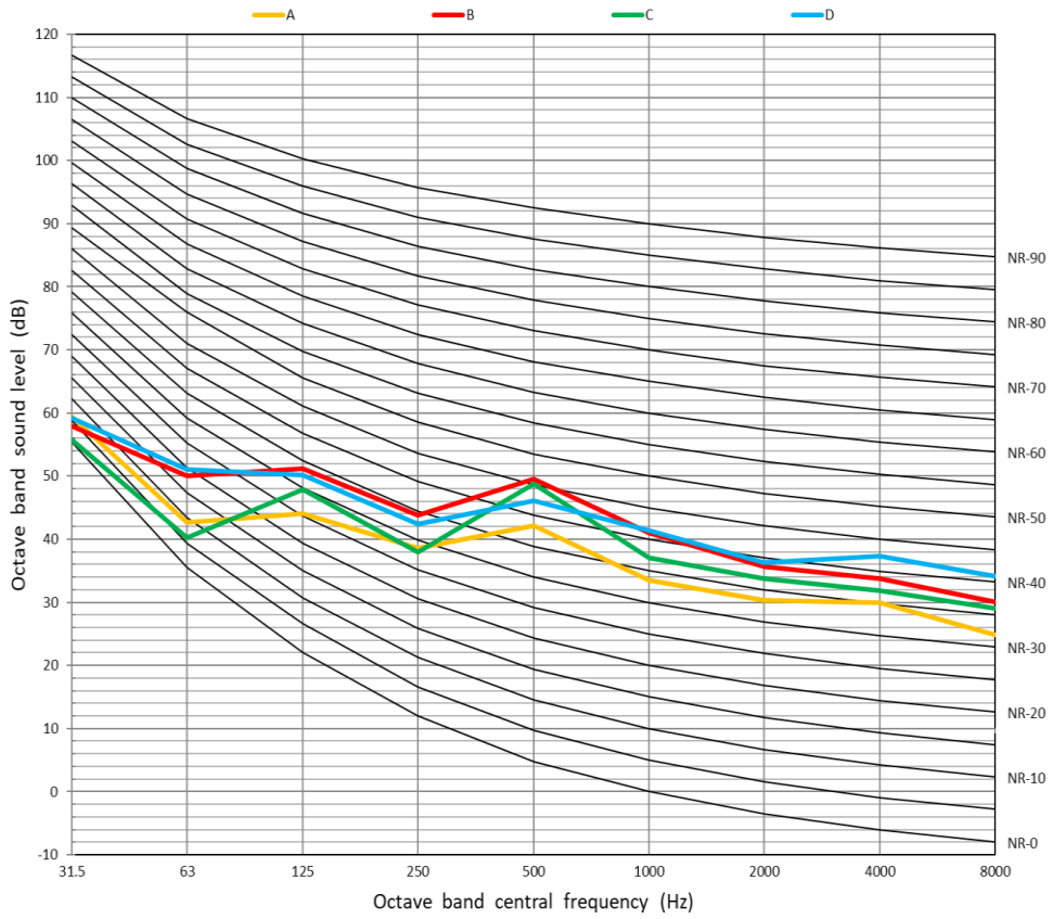
Heating A-7W35
